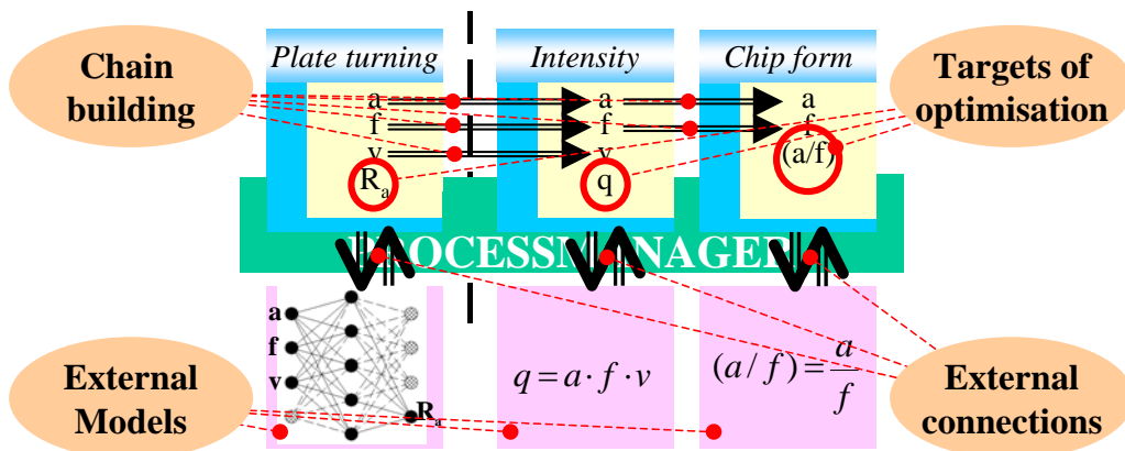
Figure 2: Hybrid modelling and optimisation by ProcessManager (model of the plate turning operation with optimisation criteria)
