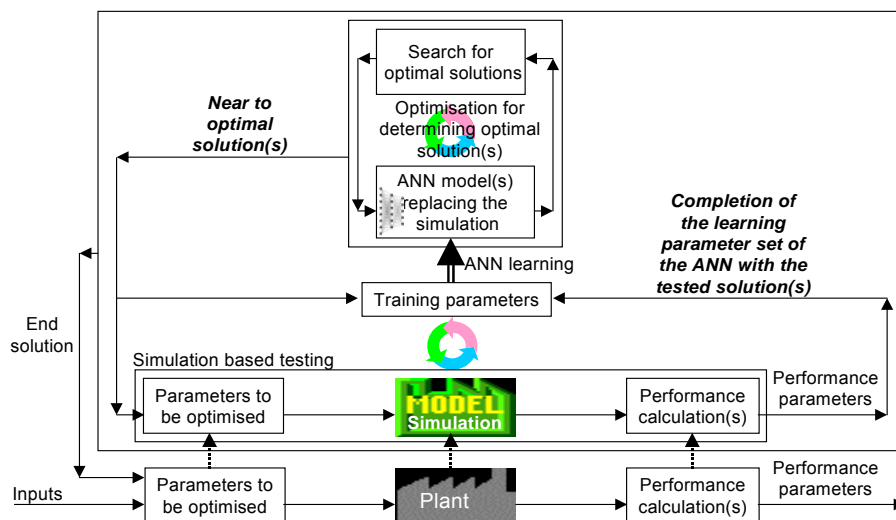
Figure 4: Concept of the hybrid, AI-, ML- and simulation-supported optimisation of production plants
