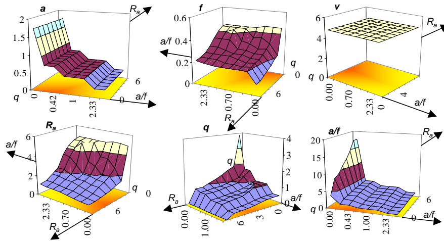
Figure 3: Parameters resulted by the threefold optimisation of the plate turning operation
