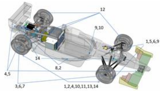
3rd diagram. Vehicle load map – categorized effects
