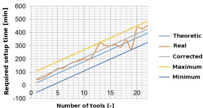
Fig. 4 Relationship of previous model and real setup times
