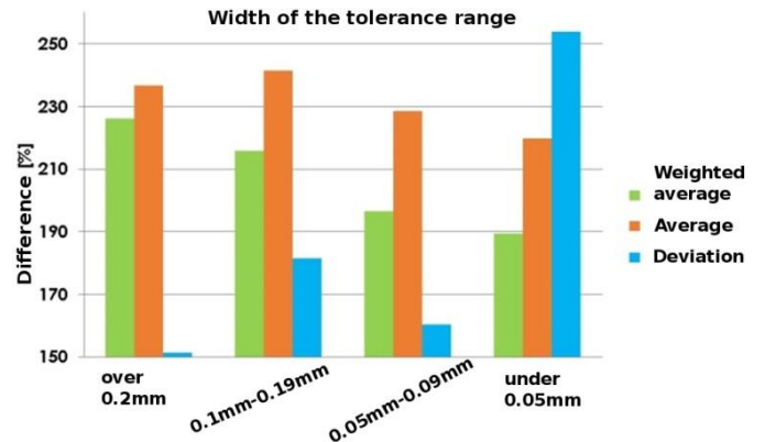
Fig. 2 Tolerance zone - time difference correlation
