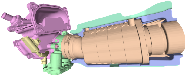
Figure 8: The assembly of the case study contains 12 components (6 screws). The coloring of the parts is similar to that in the assembly process plan (Fig. 7), except for the screws in the composite features.
