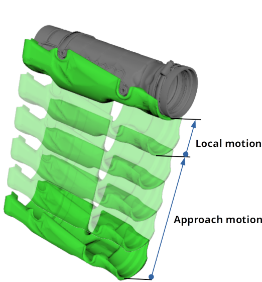
Figure 6: Illustration of X3D animation of two components being assembled, the moved component is shown in green.
