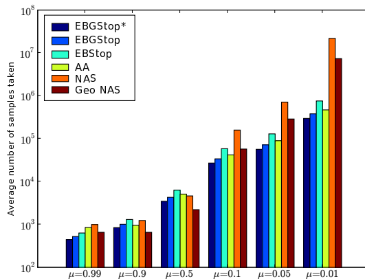
Figure 3. Comparison of stopping rules on Bernoulli random variables. The number of samples is shown in log scale.
