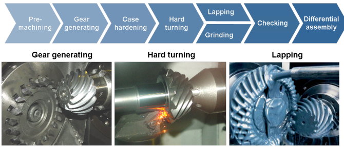
Figure 5. The BMW production process, characterized by many sensitive tolerances with complex dependencies.
