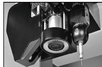
Figure 13. Multi-sensor head: laser scanner (left) and touch probe (right).
