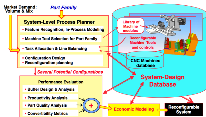
Figure 9. Integrated approach for quality oriented design of RMSs [101].
