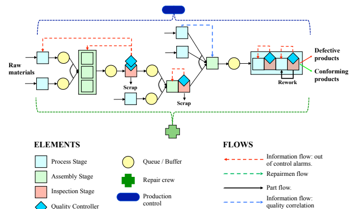
Figure 12. Representation of a manufacturing / assembly system with SPC and corrective maintenance [279].
