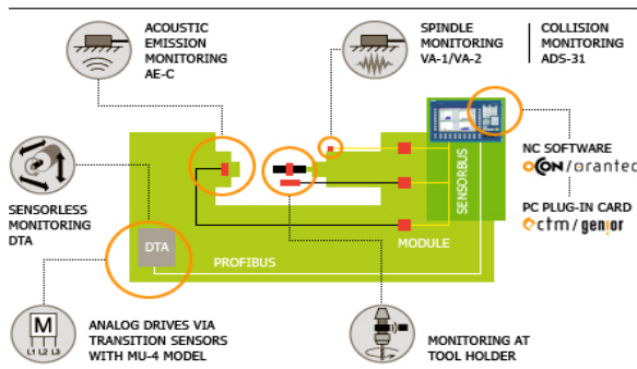
Figure 14. Multi-sensor system for process monitoring.
