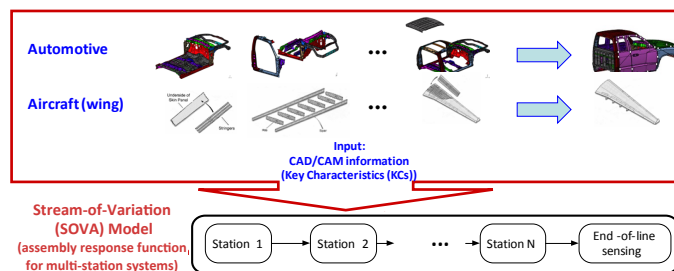
Figure 11. Main characteristics of the "Stream of Variation Analysis".
