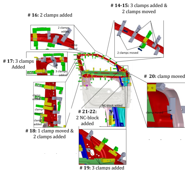
Figure 14. Engineering changes
