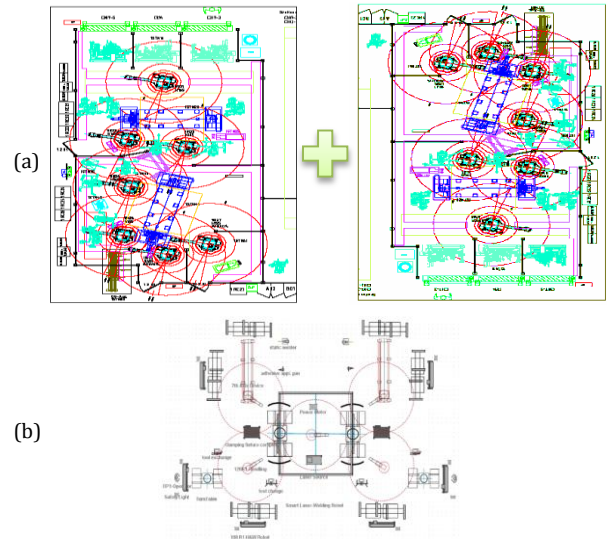
Figure 10. Current Sport Utility Vehicle: (a) RSW door assembly line for RH/LH front doors; and (b) the developed RLW cell for RH/LH doors
