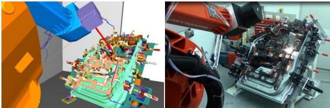
Figure 13. RLW simulated and real door fixture
