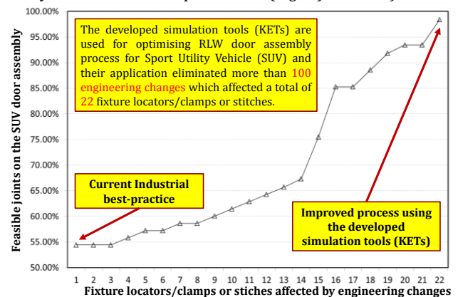
Figure 12. Simulation and optimisation based results of engineering changes to reach quality output
