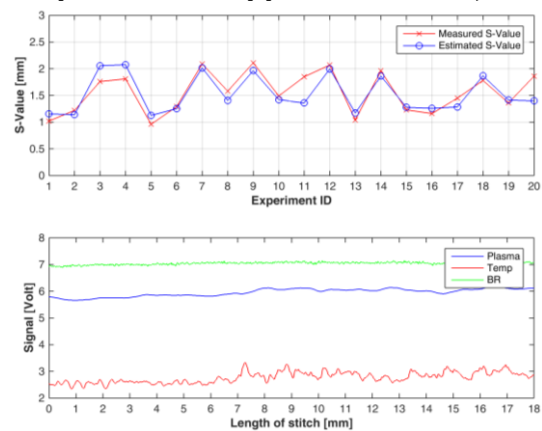
Figure 8 Signal (i.e., plasma, temperature and back-radiation) to joint performance (i.e., s-value) mapping
