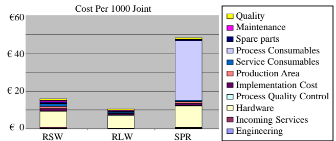
Figure 11. Cost comparison between RSW, SPR and RLW processes
