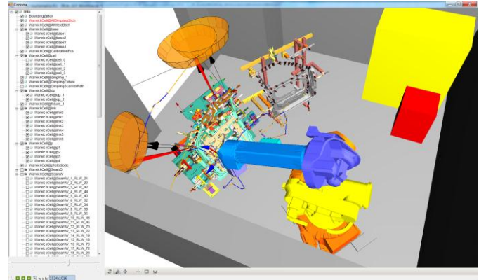
Figure 4. A completely specified RLW workcell, including a dimpling and a welding fixture.
