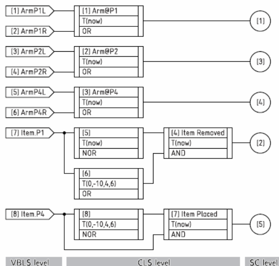
Fig. 6. The hierarchical VBLS/CLS/SC system.
