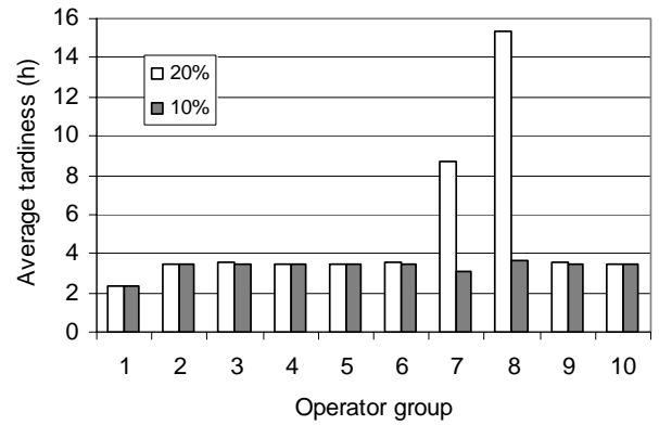
Fig. 4. The effect of missing operators: The dark bars show the results where the number of operators per group was decreased with 10% while the white bars represent the results with 20% less operator per group. The replications were carried out sequentially group by group analysing the effect of only one group at once. The results of the experiment show, that groups 7 and 8 have the main effect on the average tardiness.
