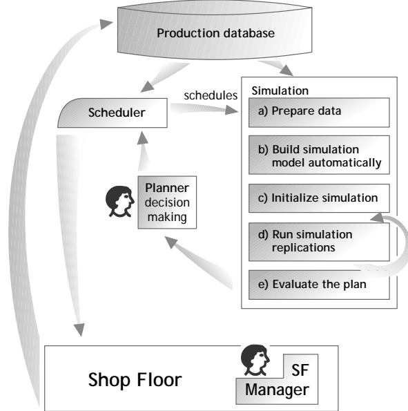
Fig. 2. Architecture and the main process flow in the simulation module
