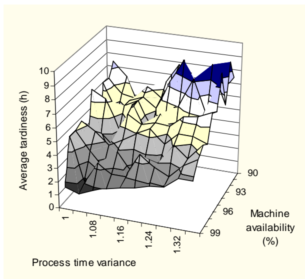
Fig. 3. The dual effect of machine availability and processing time variance on average tardiness
