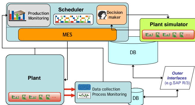
Fig. 1. Architecture for simulation-based evaluation of scheduling and rescheduling strategies, as well as the information flow in the real system
