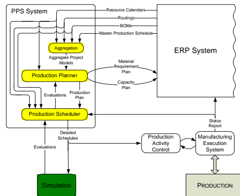
Fig. 4: Bridging the gap between ERP and MES
