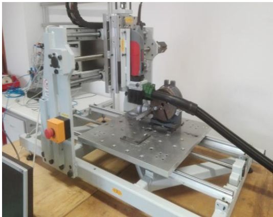
Figure 1. The applied CNC (micro-)milling machine was planned, built and it is operated in Zalaegerszeg, by the CncTeamZeg group of the Mechatronic Education and Research Institute on the Faculty of Engineering of the University of Pannonia. Originally, the machine was planned to serve with metal cutting and 3D printing operations but the preliminary calculations and the first tests on ceramic material removal proved its applicability to perform the related micro-milling of ceramics, too.
